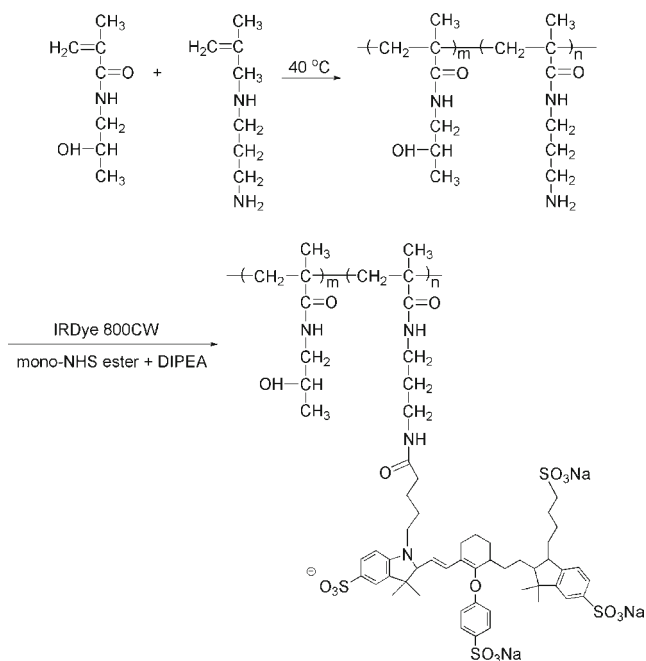
Fig. 1 The synthesis of P-IRDye.
